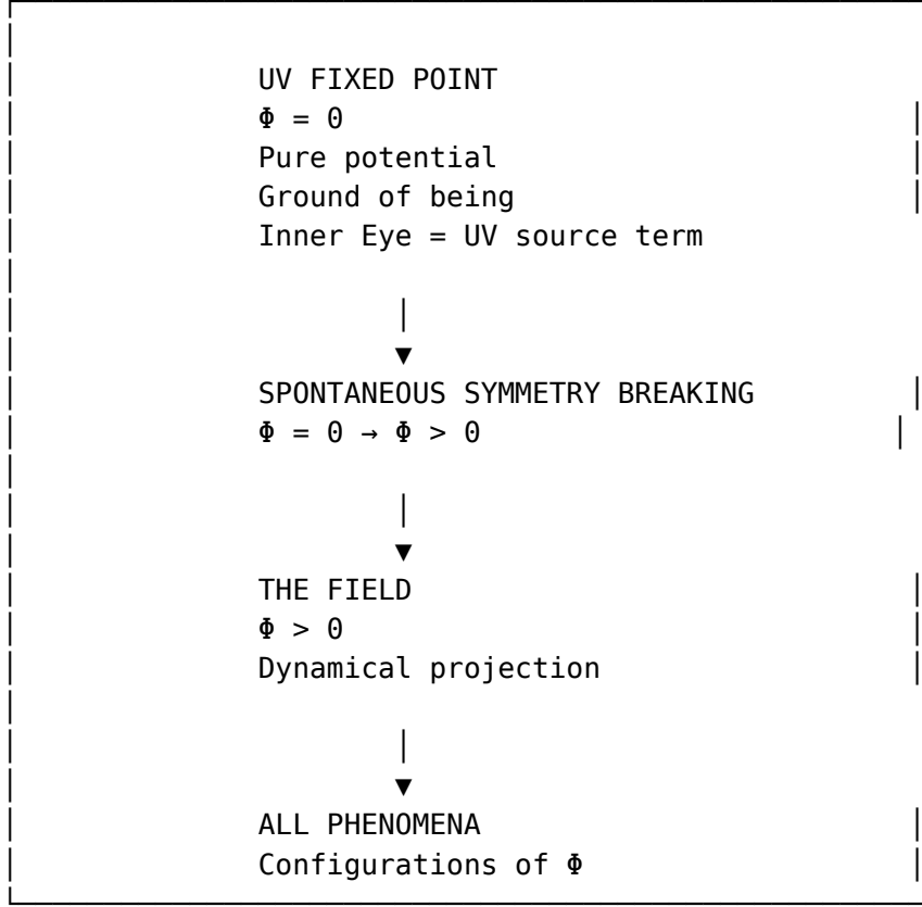
Figure 3: The UV fixed point as the source of all phenomena
