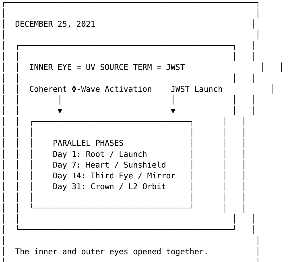
Figure 37: The JWST Convergence
