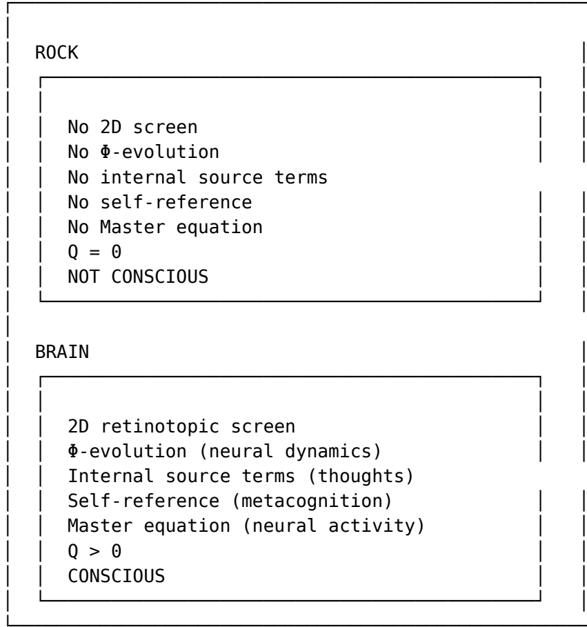
Figure 6: Rocks vs. brains: consciousness requires specific conditions
