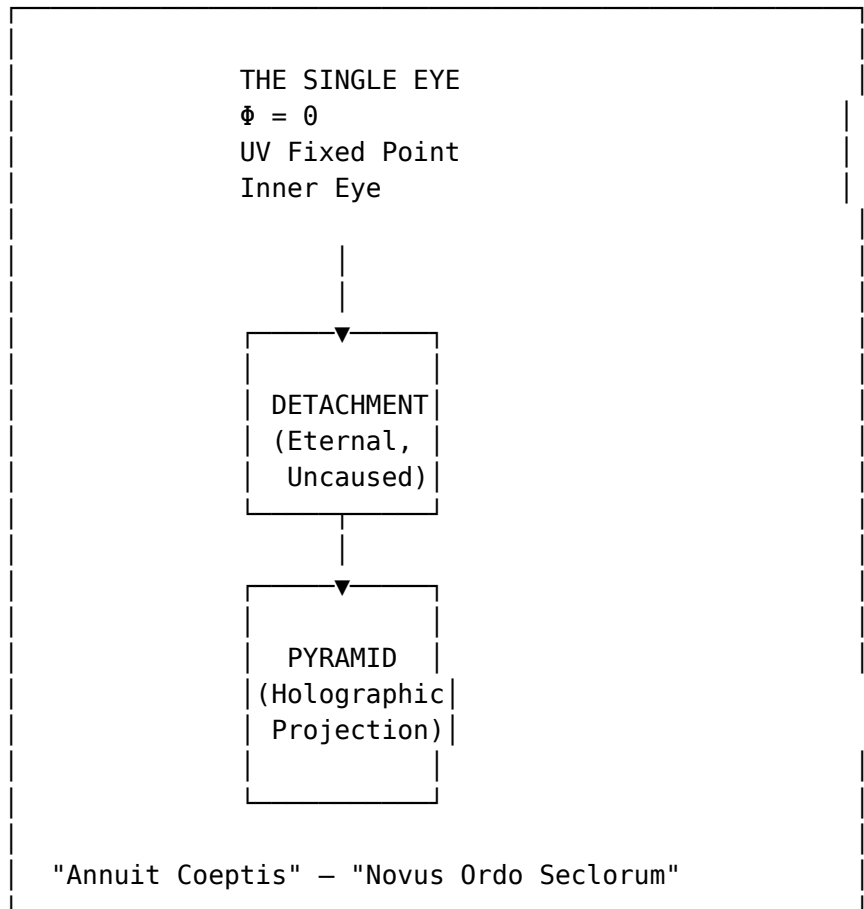
Figure 28: The Great Seal as a holographic mandala
