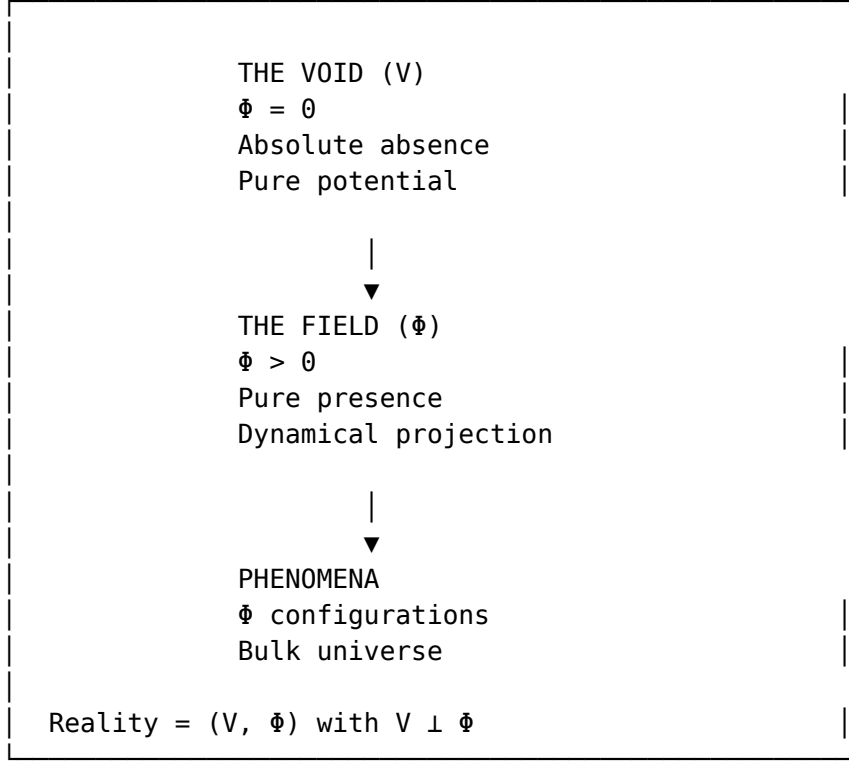
Figure 1: The dual-aspect ontology of the Void and the Field
