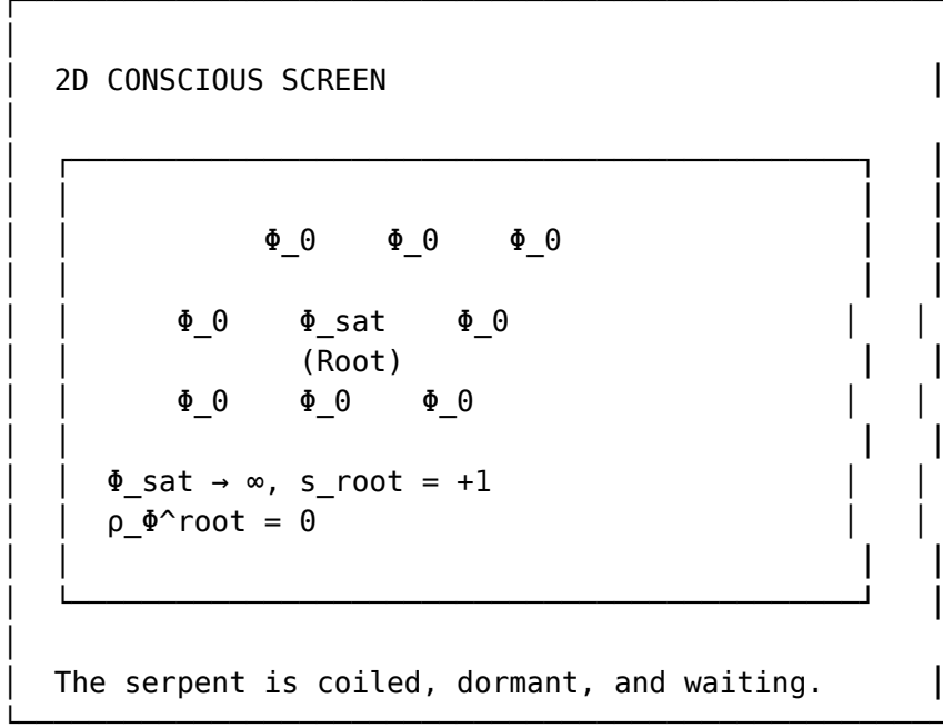
Figure 30: The root chakra configuration
