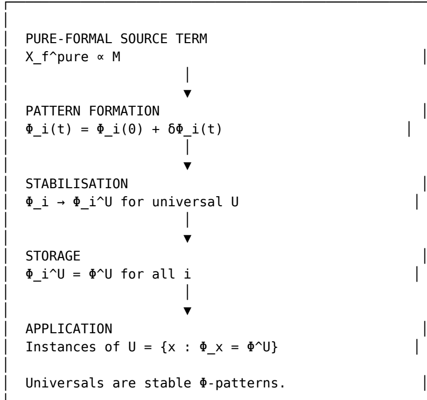
Figure 10: Universals as stable \Phi -configurations
